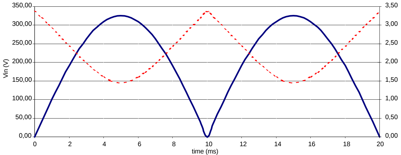
Figure 57. Input Voltage and On-time vs Time (example with F_{SW} = 100 \text{ kHz} , P_{in} \approx 150 \text{ W} , V_{AC} = 230 \text{ V} , L = 200 \mu\text{H} )
