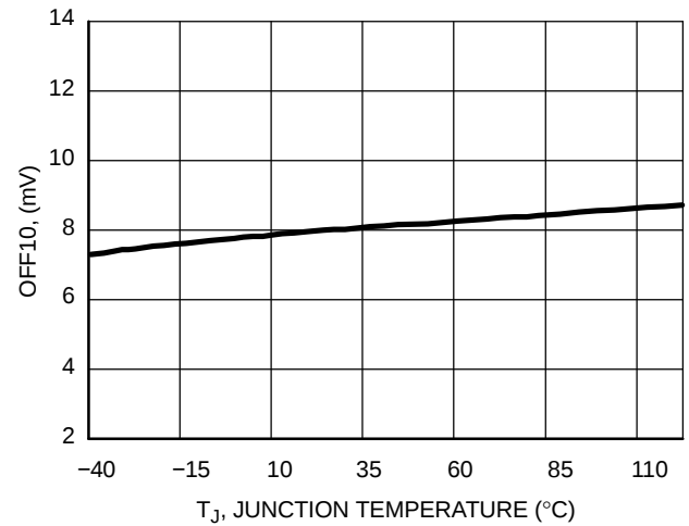
Figure 39. Current Sense Pin Voltage vs. Temperature (10 \mu A Being Drawn from Pin 5)
