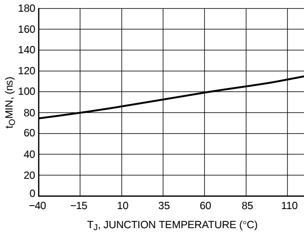
Figure 48. Minimum On-Time vs. Temperature
