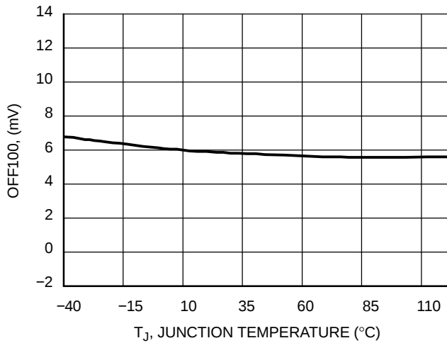
Figure 38. Current Sense Pin Voltage vs. Temperature (100 \mu A Being Drawn from Pin 5)
