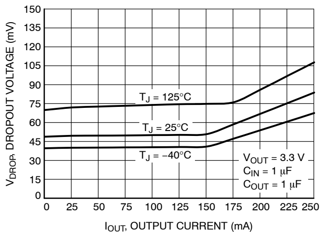
Figure 18. Dropout Voltage vs. Load Current – V_{OUT} = 3.3\text{ V}
