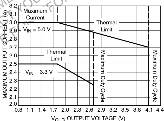
Figure 27. Derating Curves
