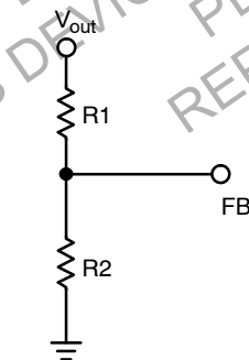
Figure 25. Output divider
