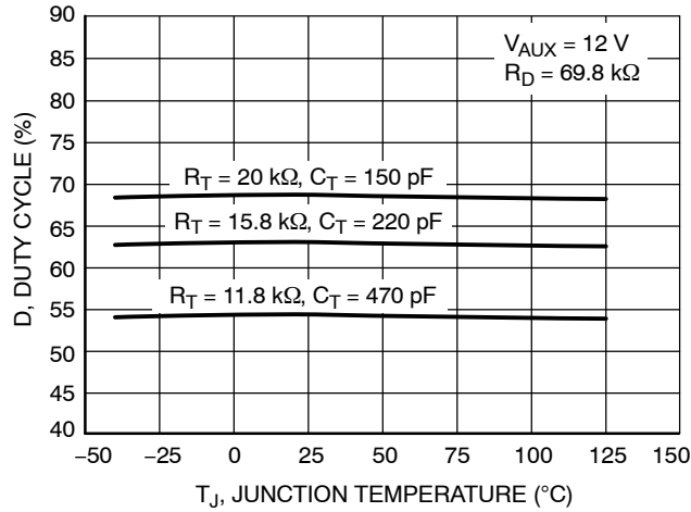
Figure 26. Duty Cycle vs. Junction Temperature
