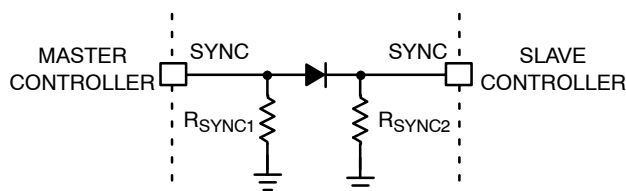
Figure 50. Master-Slave Configuration
