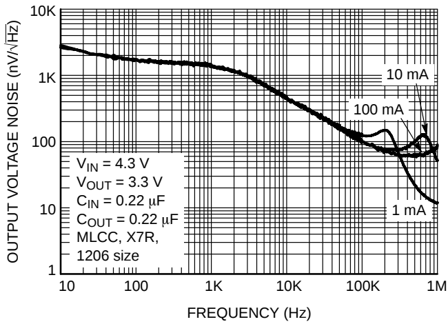
Figure 28. Output Voltage Noise Spectral Density for V_{OUT} = 3.3 \text{ V} , C_{OUT} = 220 \text{ nF}
