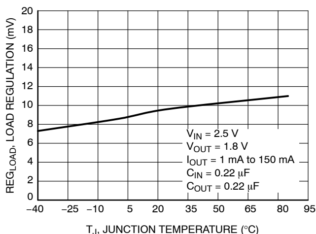
Figure 10. Load Regulation vs. Temperature V_{OUT} = 1.8\text{ V}
