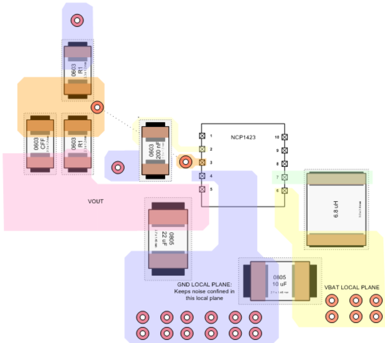
Figure 33. Layout Guidelines
