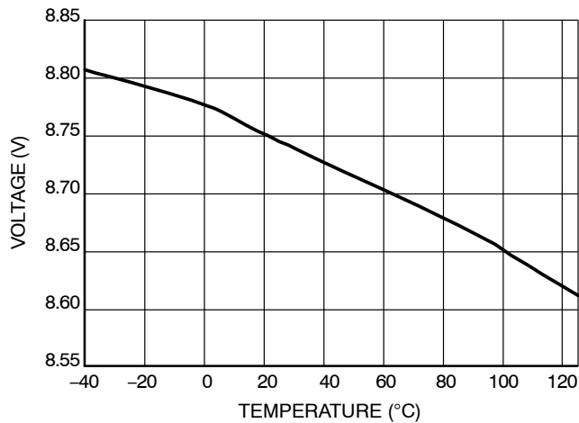
Figure 6. V_{BOOTon}
