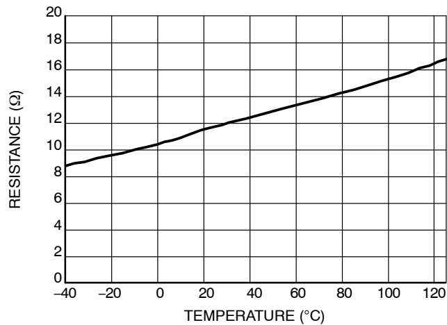
Figure 8. R_{OH}
