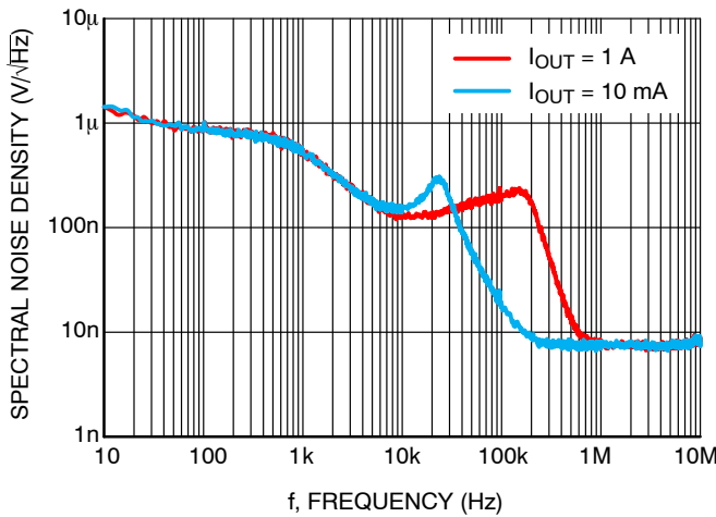
Figure 10. Output Voltage Spectral Noise Density vs. Frequency – V_{OUT(NOM)} = 1.0\text{ V}
