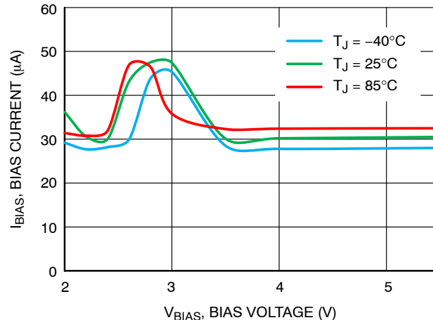
Figure 7. BIAS Pin Current vs. V_{BIAS} and T_J
