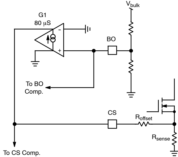
Figure 20. A Transconductance Amplifier Transforms the BO Voltage into a Current
