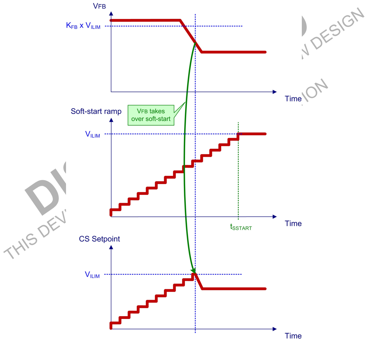
Figure 57. Soft-Start Feature
