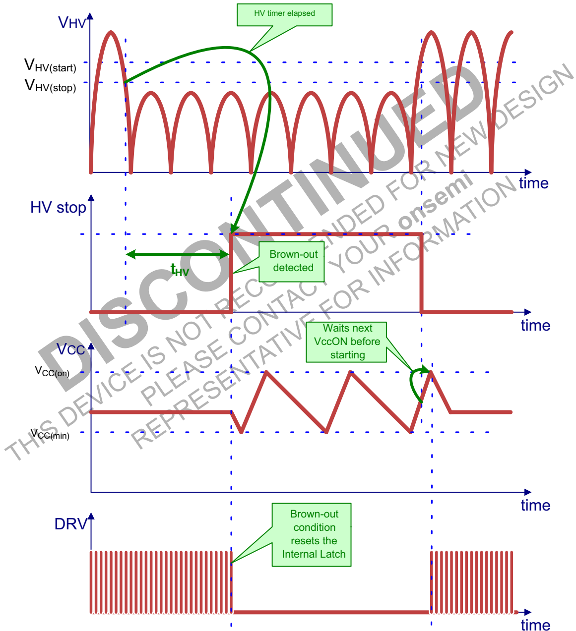
Figure 46. Ac Line Drop-out Timing Diagram
