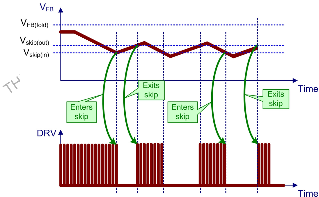
Figure 56. Skip Mode Timing Diagram
