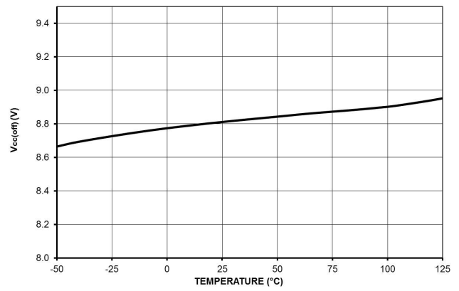
Figure 27. V CC Turn-off Threshold (UVLO) V CC (off)
