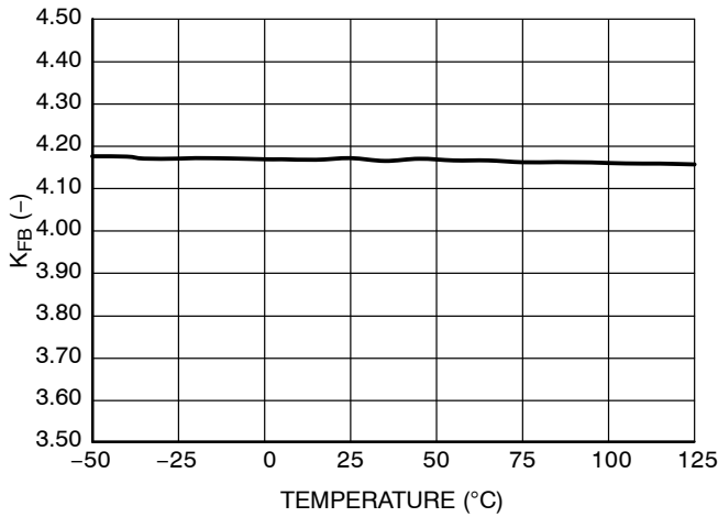
Figure 17. V_{FB} to Internal Current Setpoint Division Ratio K_{FB}
