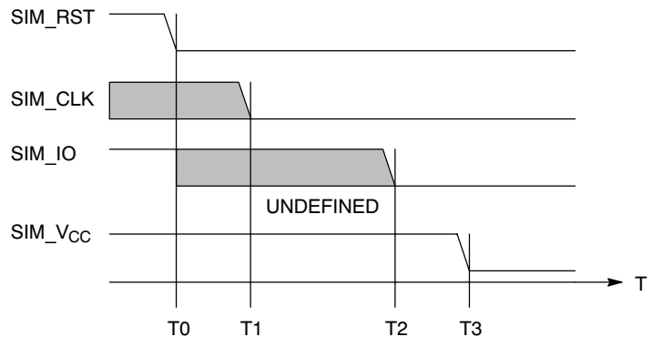
Figure 4. ISO7816-3 Power Down Sequence
