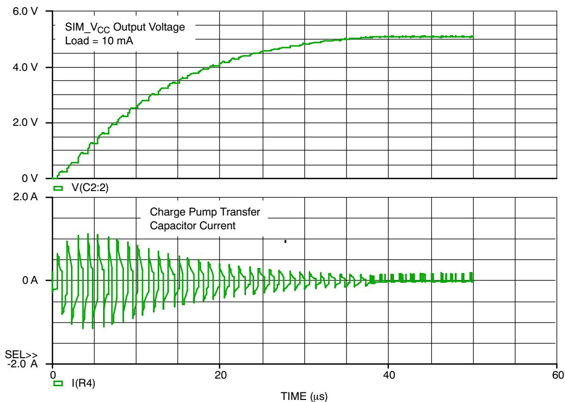
Figure 12. Simulated Charge Pump Typical Waveforms
