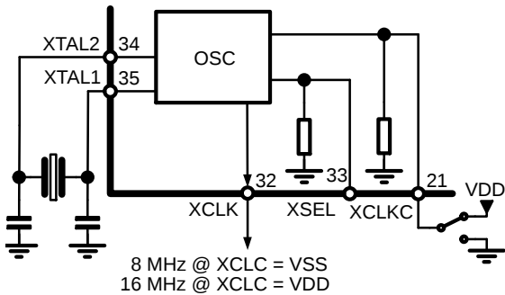
Figure 16. XTAL Oscillator
