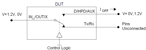
Figure 16. Off State Leakage
