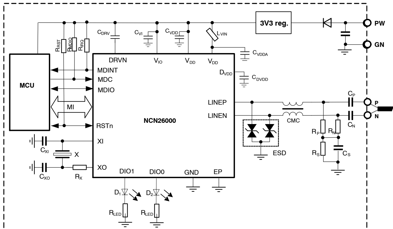
Figure 6. Application Diagram
