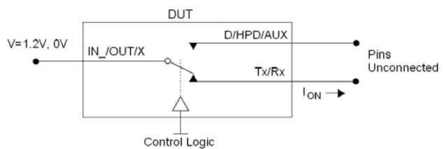
Figure 15. On State Leakage
