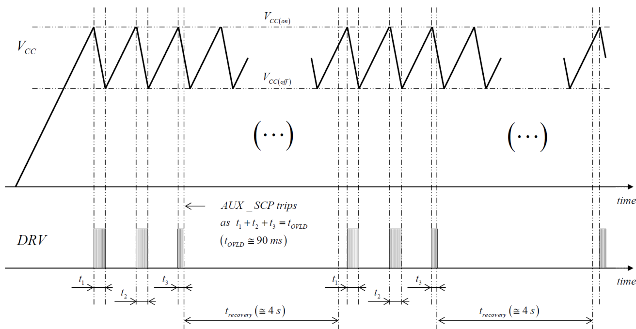
Figure 5. Start-up Sequence in a Load Short-circuit Situation
