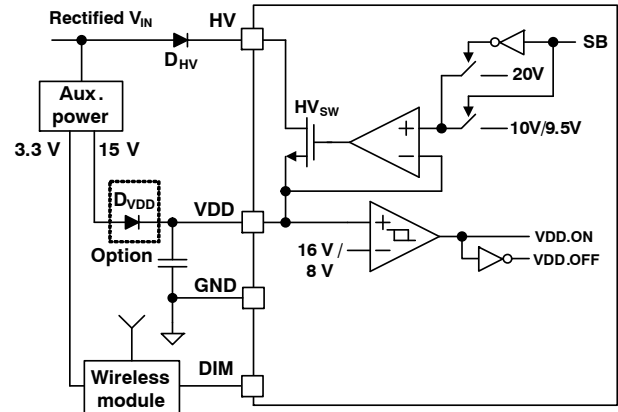
Figure 14. VDD Supply
