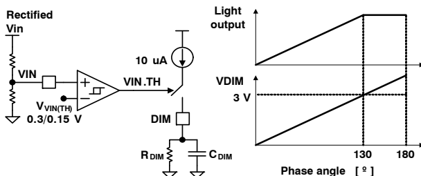
Figure 13. PCDIM Operation
