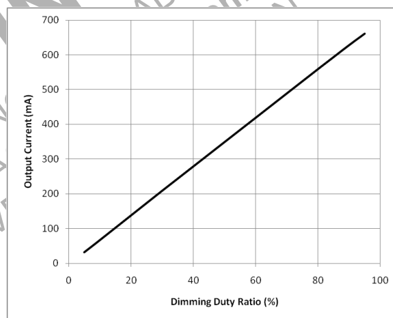
Figure 8. Dimming Performance
