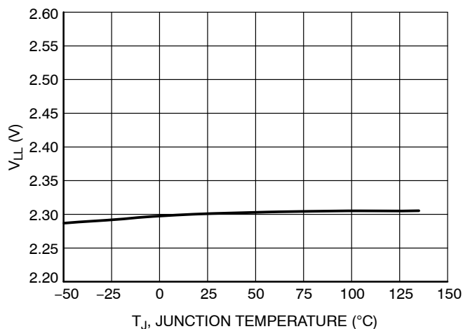
Figure 40. Threshold for Low-line Range Detection vs. Temperature
