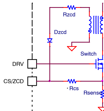
Figure 8. ZCD Winding Implementation
