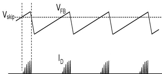
Figure 56. Soft-Skip Operation
