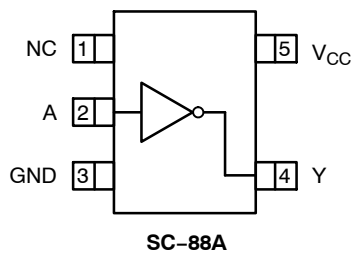
Figure 1. Pinout Diagrams (Top Views)
