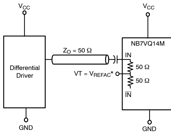
Figure 15. Capacitor-Coupled Single-Ended Interface ( V_T Connected to V_{REFAC} )
