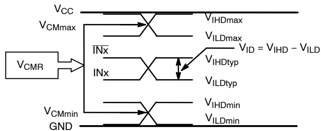
Figure 9. V_{CMR} Diagram
