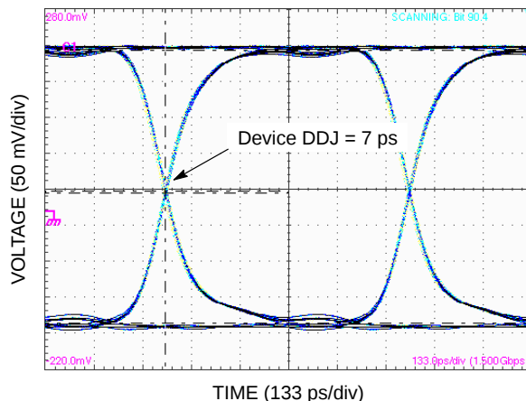
Figure 1. Typical Output Waveform at 1.5 Gb/s with K28.5 (V_{INPP} = 100\text{ mV}, \text{Input Signal DDJ} = 24\text{ ps})
