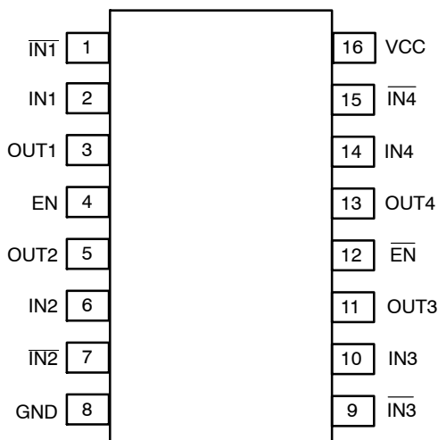
Figure 2. TSSOP-16 Pinout (Top View)
