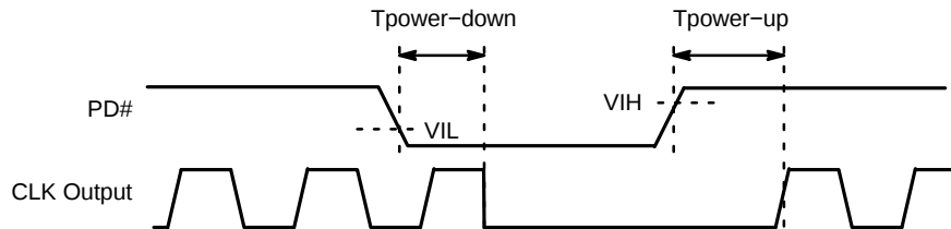
Figure 8. Output Enable/Disable and Power Down Functions
