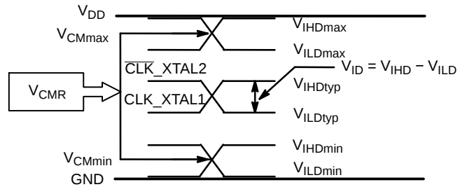
Figure 7. V_{CMR} Diagram
