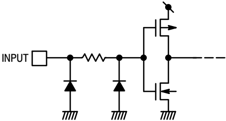
Figure 4. Input Equivalent Circuit
