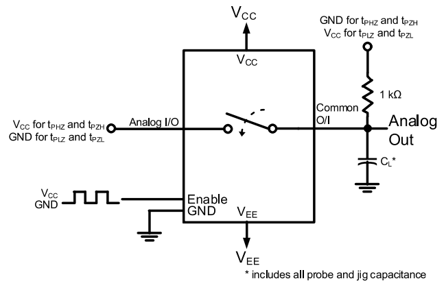
Figure 14. Propagation Delay, Enable to Analog Out
