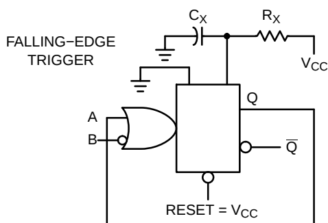
Figure 14. Non-retriggerable Monostable Circuitry
