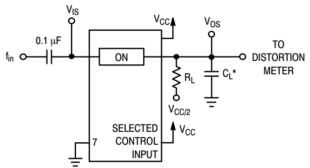
Figure 19. Total Harmonic Distortion Test Setup
