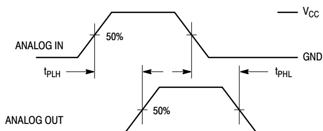
Figure 10. Propagation Delay, Analog In to Analog Out
