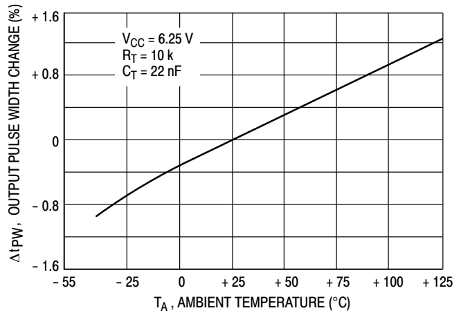
Figure 4. f_{out} , Pulse Width Change versus Temperature
