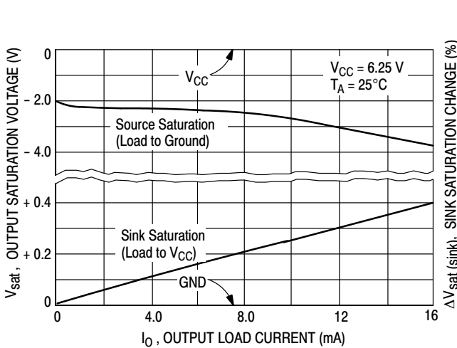
Figure 7. f_{out} , Saturation versus Load Current
