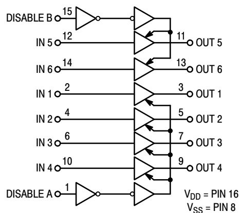
LOGIC DIAGRAM
