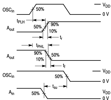
Figure 1. Switching Waveforms
