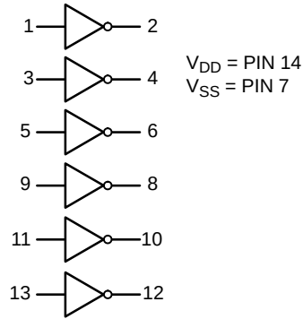
Figure 1. Logic Diagram
