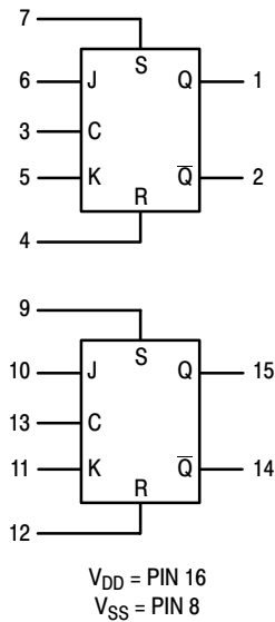
BLOCK DIAGRAM
