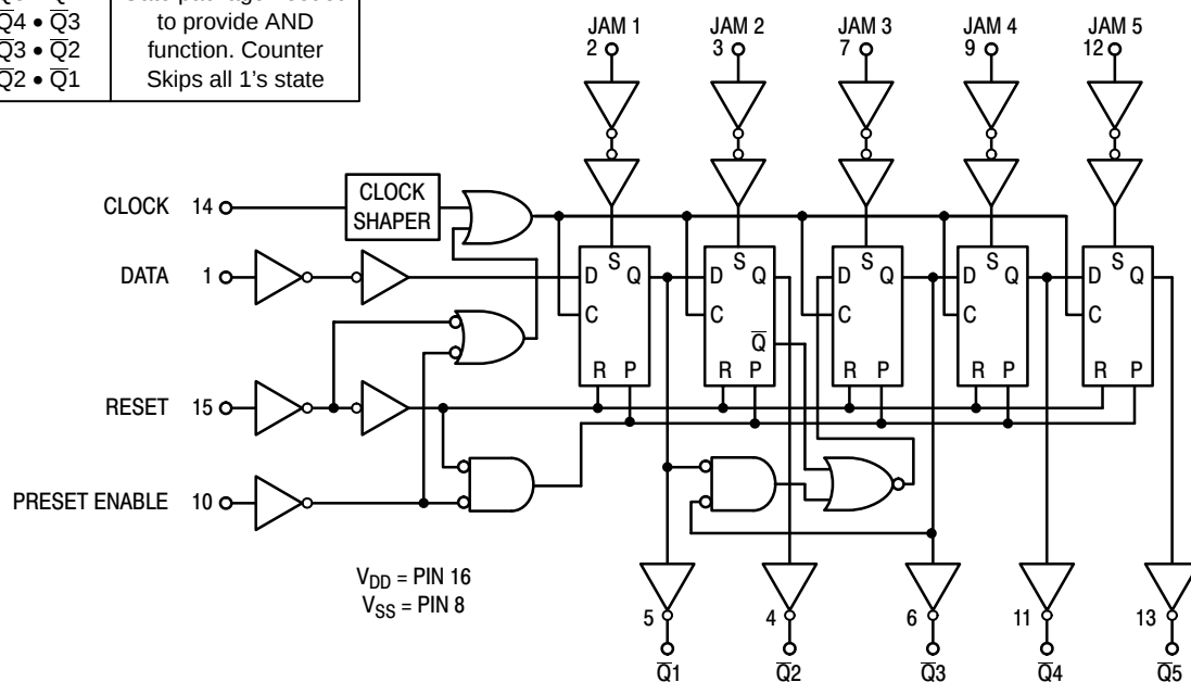
LOGIC DIAGRAM
