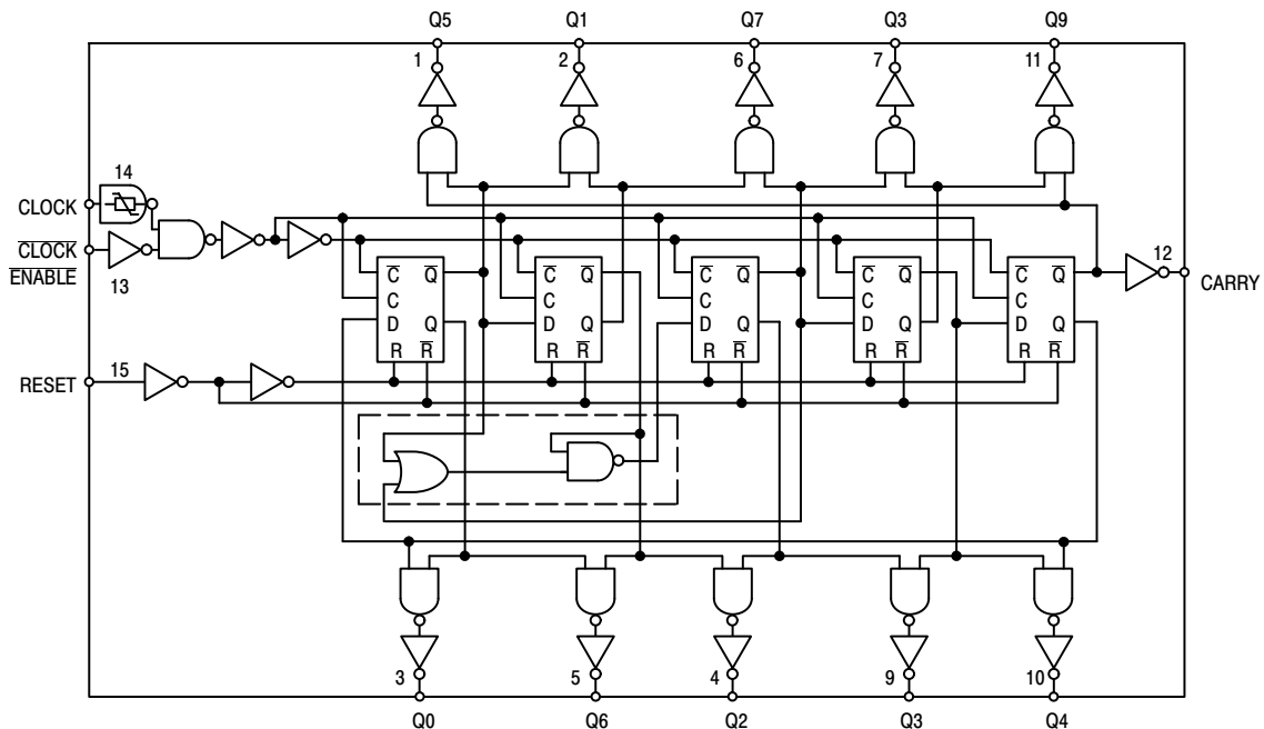
LOGIC DIAGRAM
