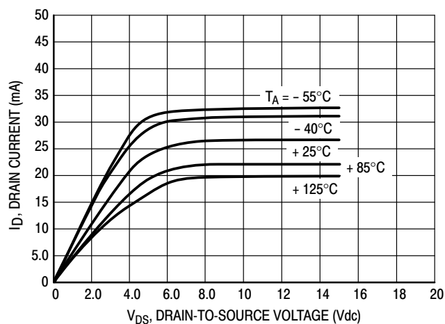
Figure 6. V_{GS} = 15 Vdc
