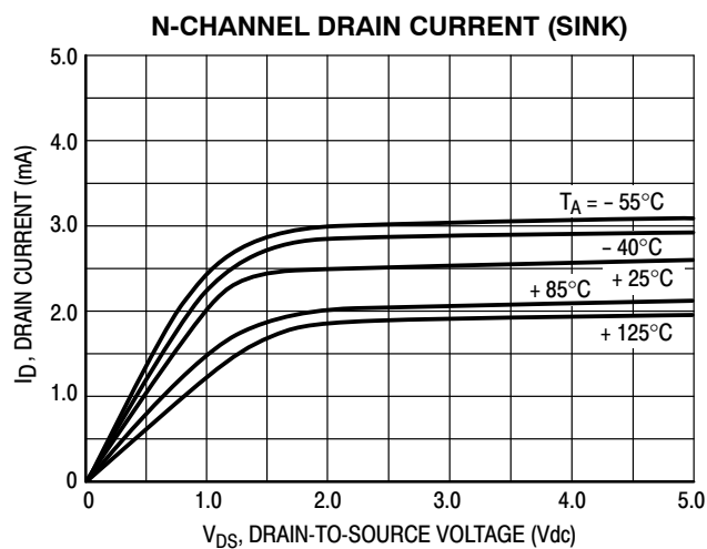
Figure 2. V_{GS} = 5.0 Vdc
