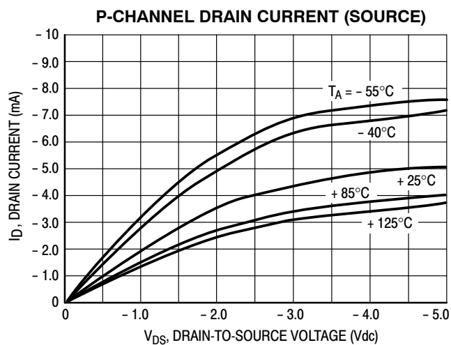
Figure 3. V_{GS} = -5.0 Vdc
