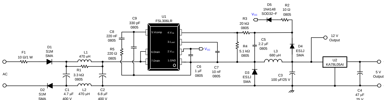
Figure 31. Schematic
