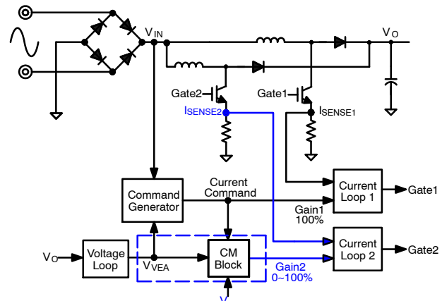
Figure 10. Current Balance Factors
