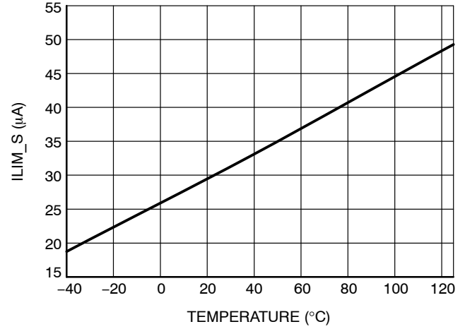
Figure 19. 30 \mu\text{A} Current Source for Current Limit Purpose vs. T at V_{HVBias} = 48\text{ V}
