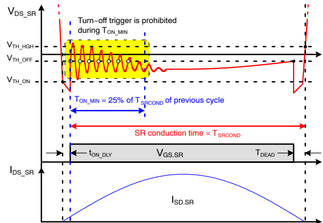
Figure 25. Minimum Turn-on Time
