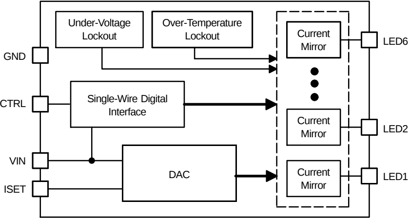
Figure 4. Block Diagram
