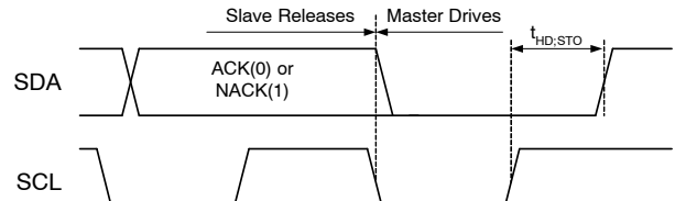
Figure 20. STOP Bit
