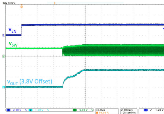
Figure 11. V_{OUT} Change: Forced PT to BOOST
