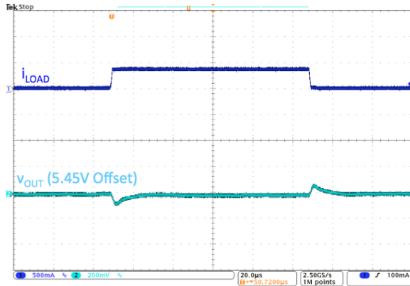
Figure 9. Load Transient, 10 ↔ 400 mA, 1 \mu\text{s} Edge
